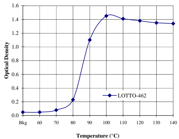
Static Sensitivity
