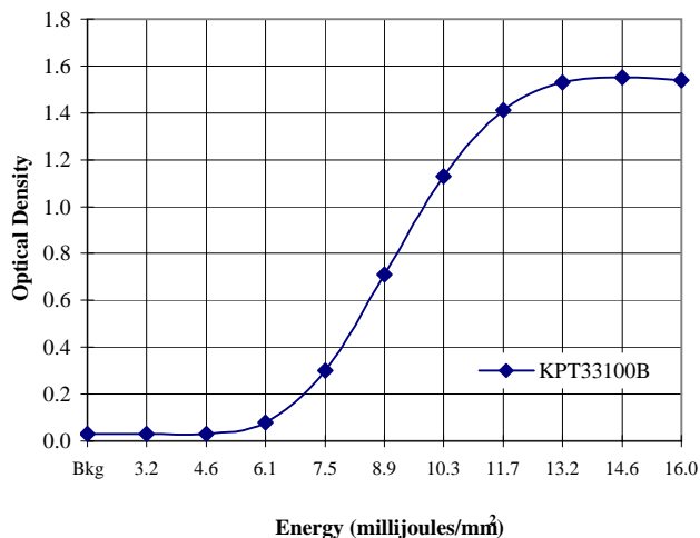
Dynamic Sensitivity
