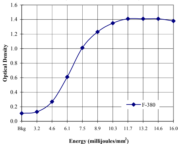
Dynamic Sensitivity
