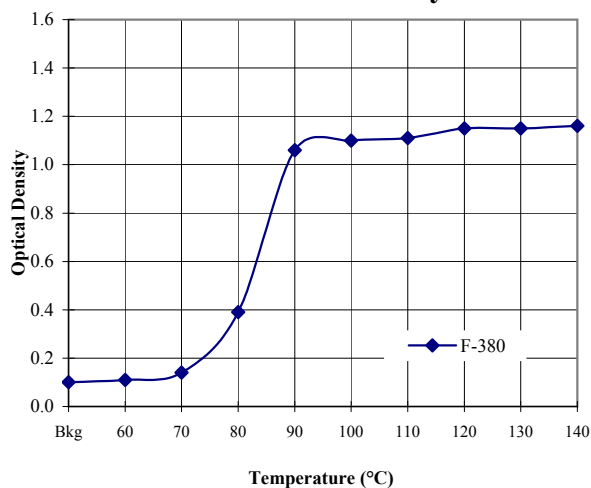
Static Sensitivity
